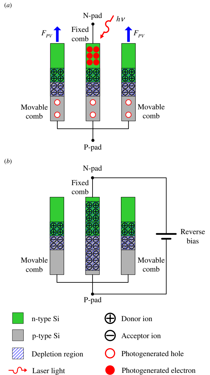
Figure 2. Driving principles of the pn-combs, (a) optical driving by the photovoltaic effect, and (b) electrical driving by applying a reverse bias.
